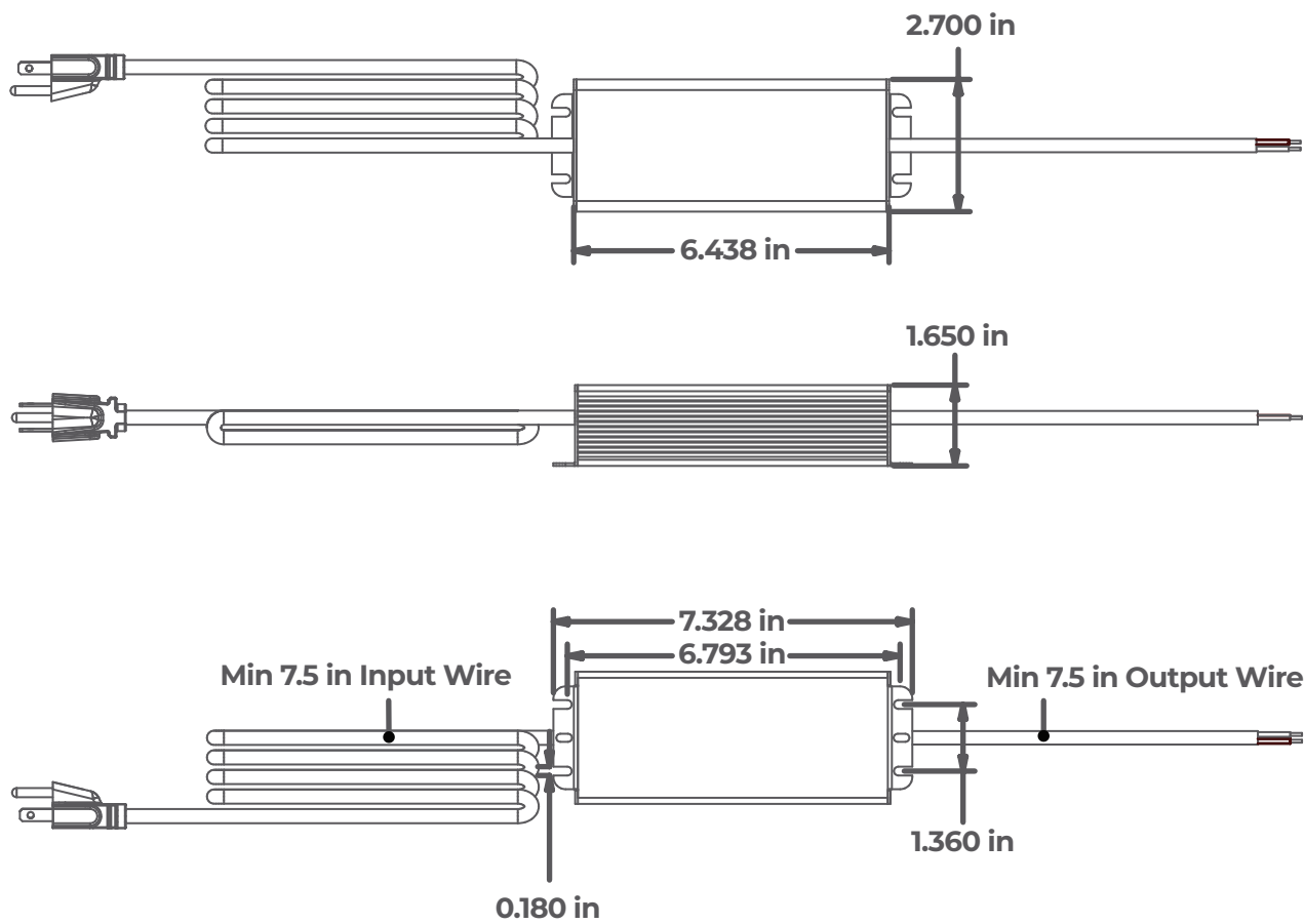
100 Watt LED Power Supply AL-PS-W-100-24
