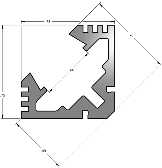
Surface Mount LED Channel, Narrow AL-TRK-SM-N
