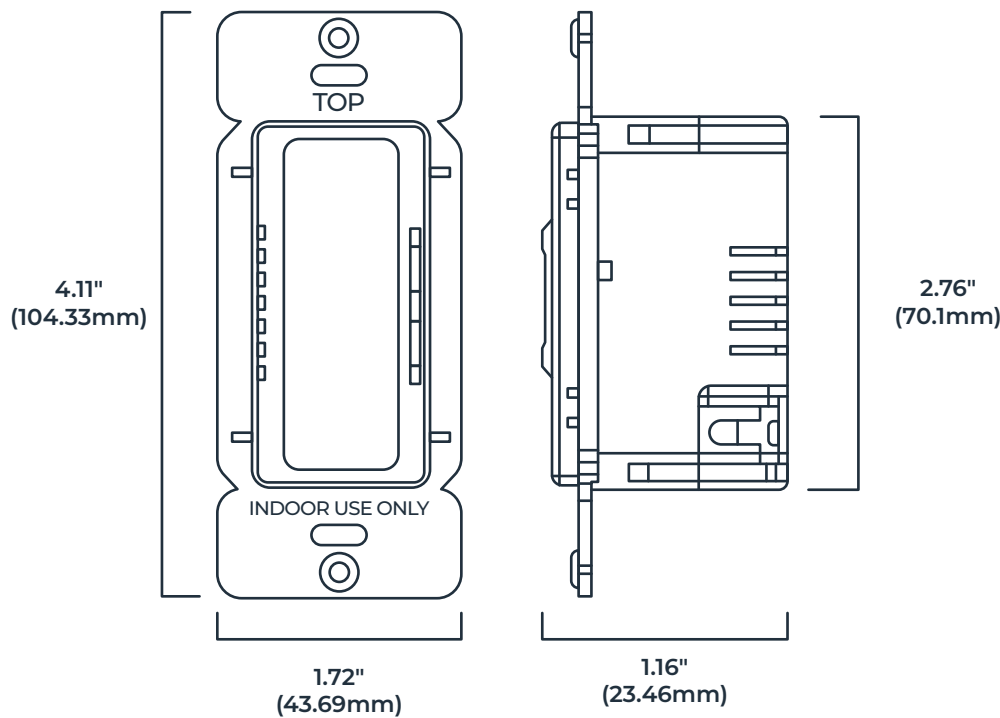
Casambi In-Wall Wireless Dimmer Switch AL-CTLR-DIMSW-CAS
