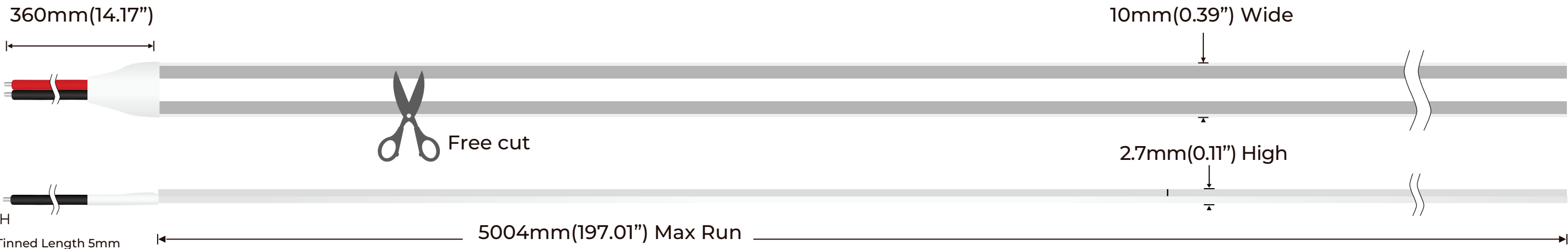
Summit LED Strip Light – Free Cut, 3000K AL-SL-FC-IP20-24-3K
