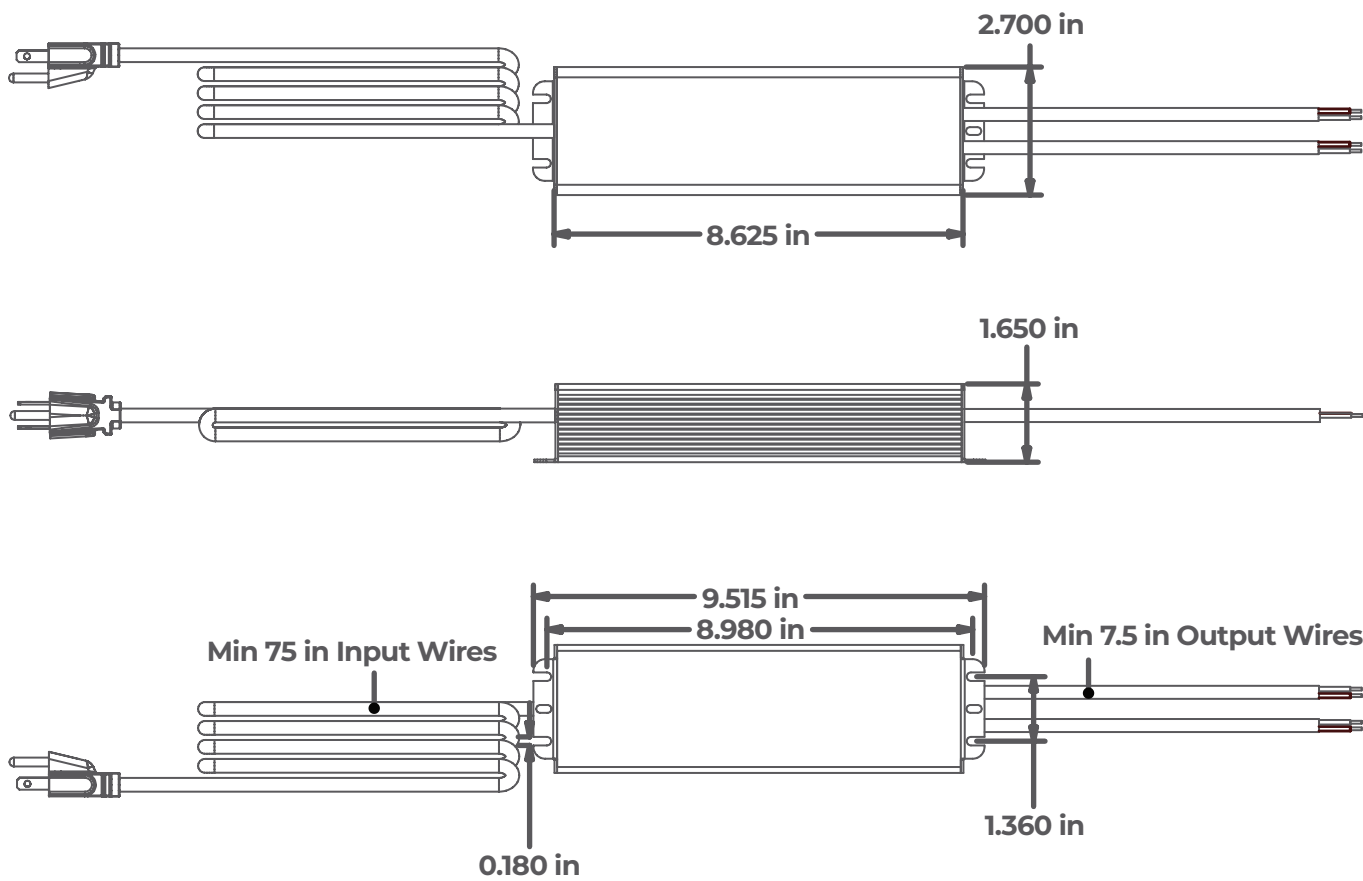
150 Watt LED Power Supply AL-PS-W-150-24
