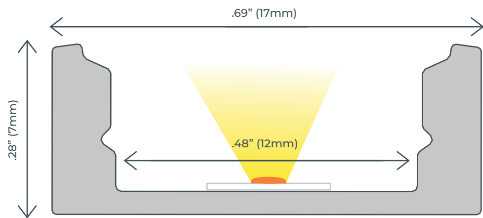
Surface Mount LED Channel, Narrow AL-TRK-SM-N
