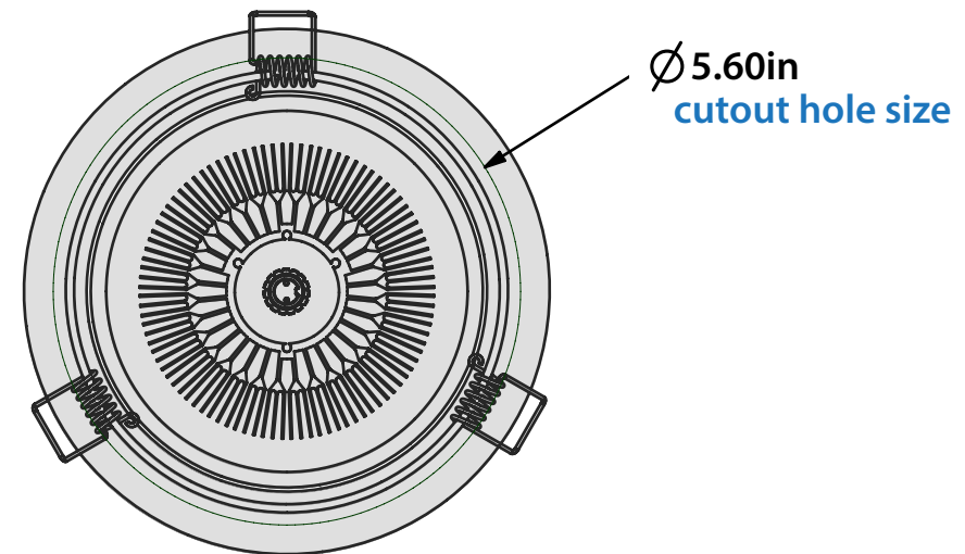
BOTTOM VIEW
