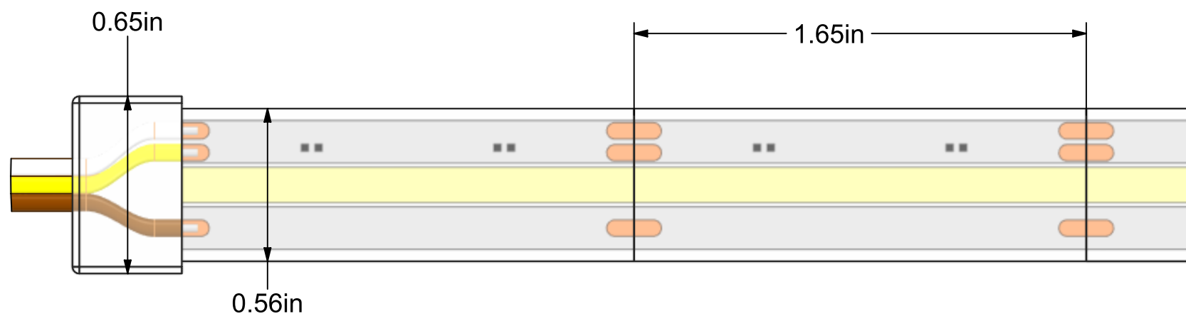
DETAIL A SCALE 2:1
