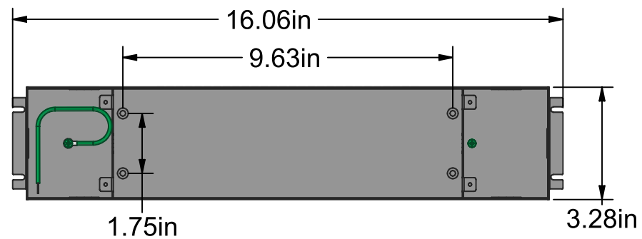
TOP VIEW LID NOT SHOWN TO SHOW INTERNAL FEATURES
